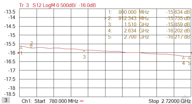
【图3】插入损耗 Insertion Loss
