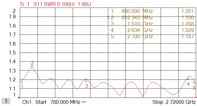
【图1】合路端驻波比InPut Port VSWR
